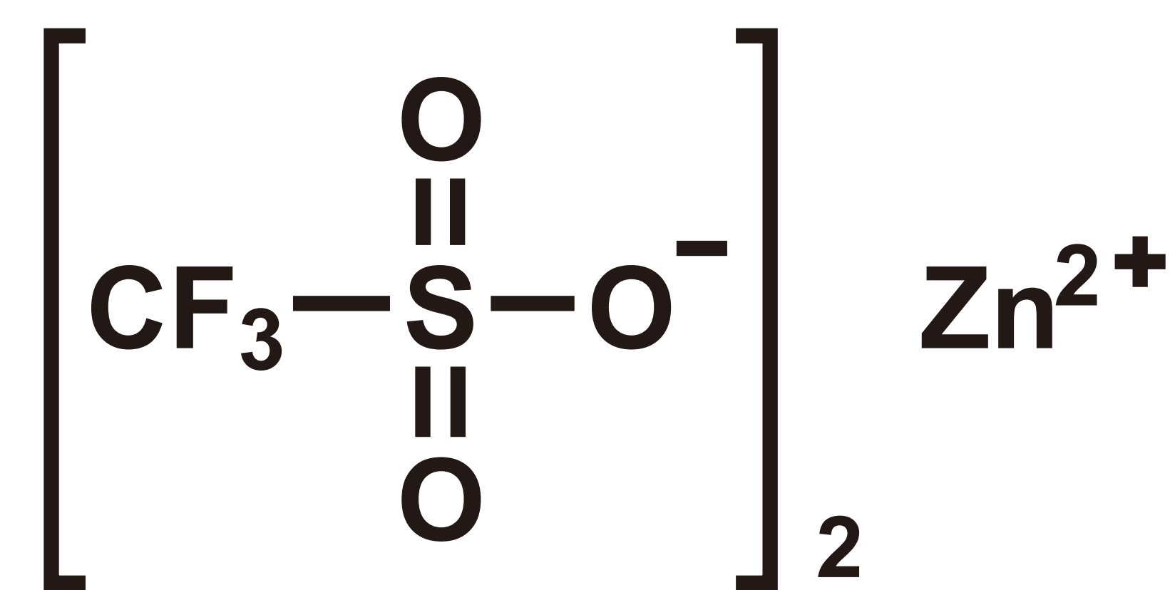
Zinc(II) Triflate [CAS RN: 54010-75-2]
