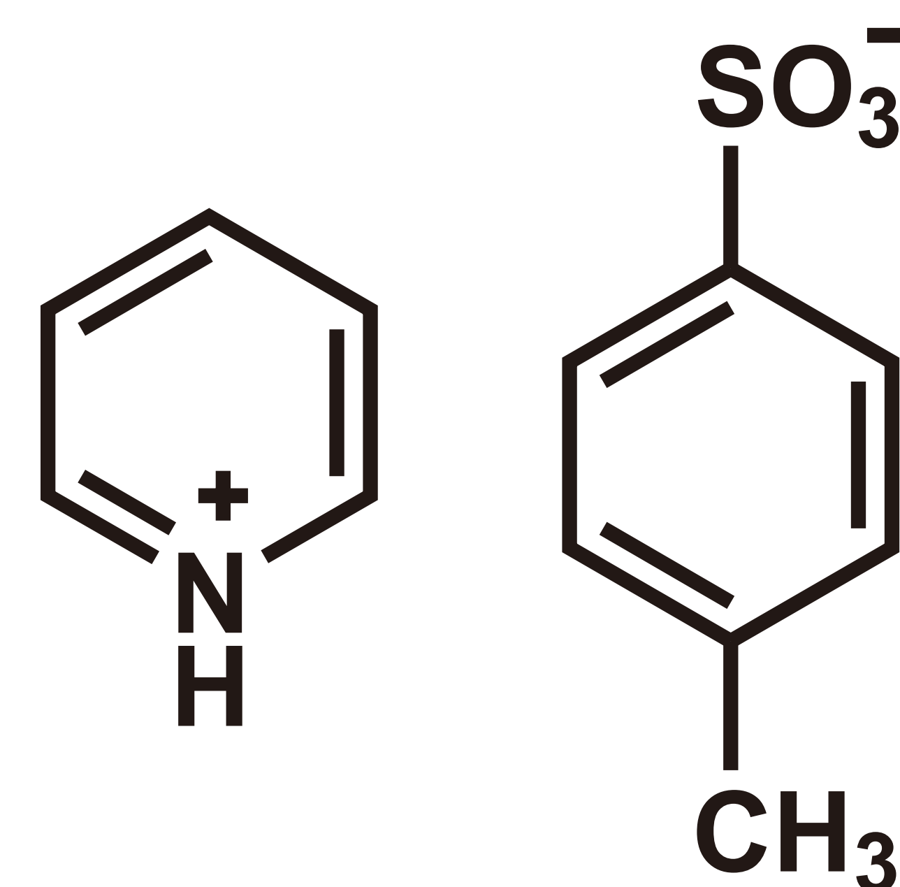
Pyridinium p-Toluenesulfonate (= PPTS) [CAS RN: 24057-28-1]
