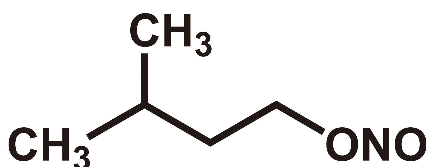
Isoamyl Nitrite [CAS RN: 110-46-3]
