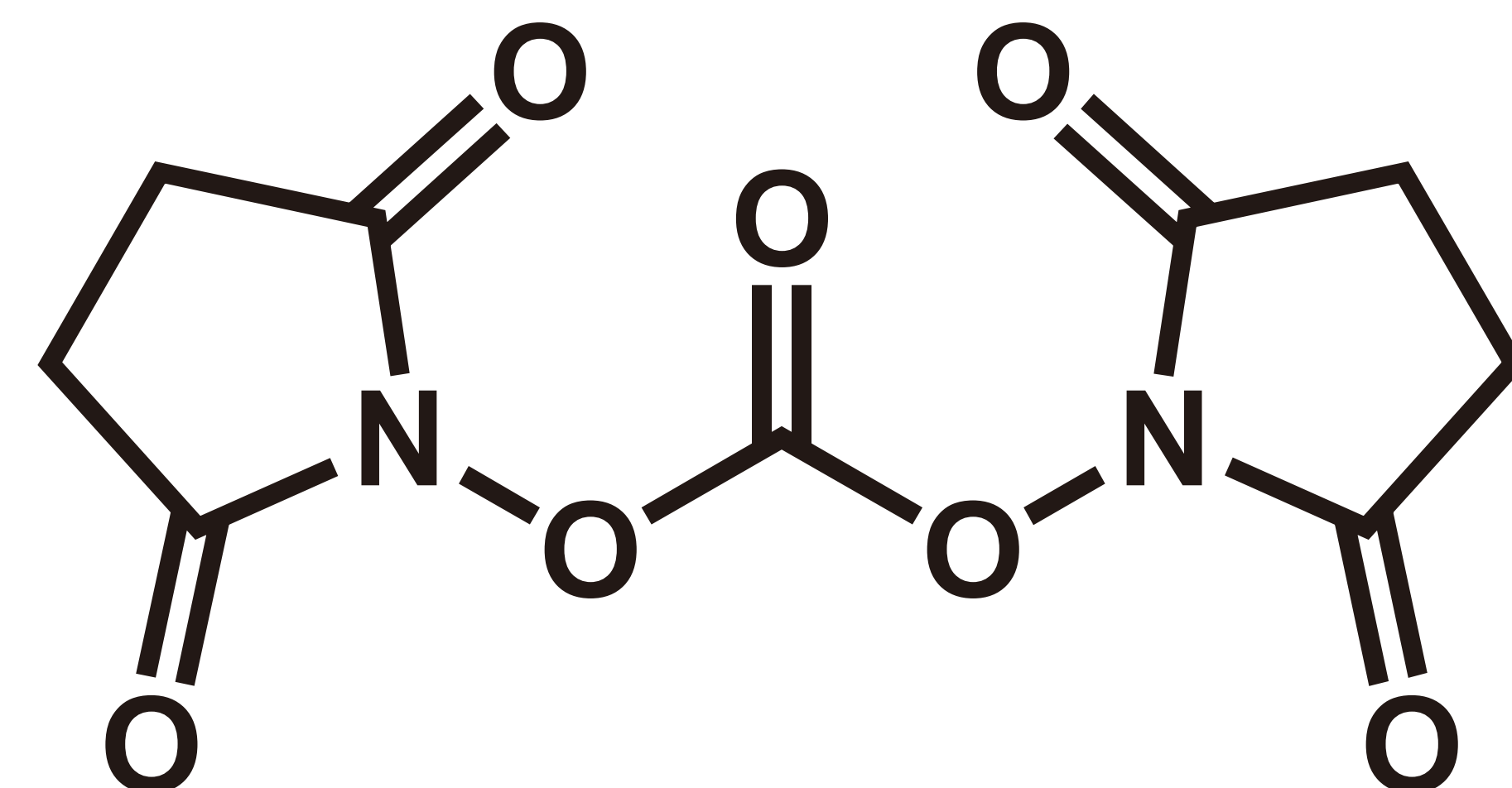
Di(N-succinimidyl) Carbonate (= DSC) [CAS RN: 74124-79-1]
