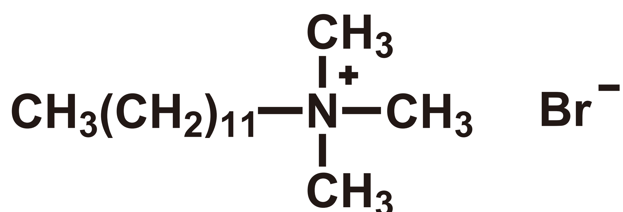
Dodecyltrimethylammonium Bromide (= DTAB) [CAS RN: 1119-94-4]
