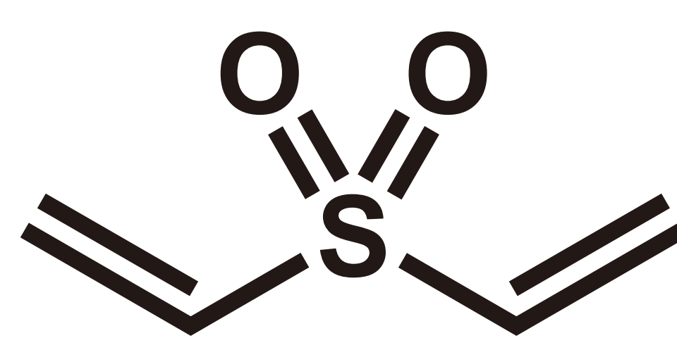
Divinyl Sulfone [CAS RN: 77-77-0]
