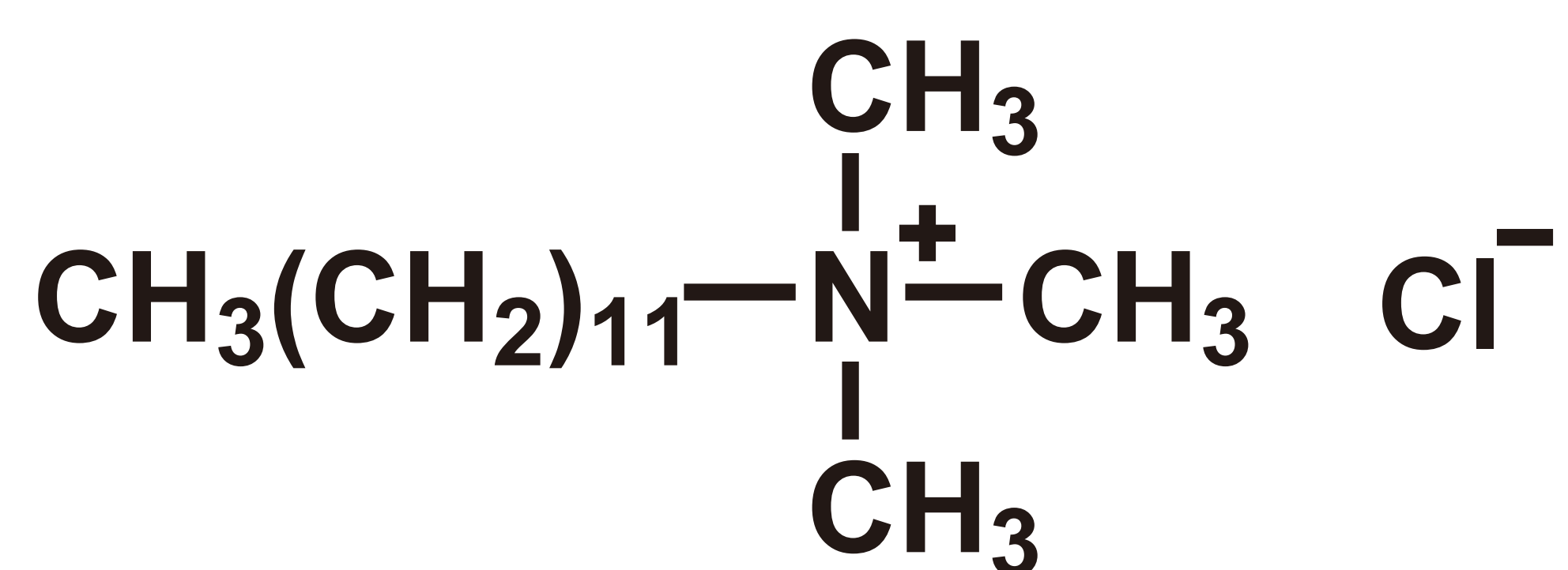
Dodecyltrimethylammonium Chloride (= DTAC) [CAS RN: 112-00-5]
