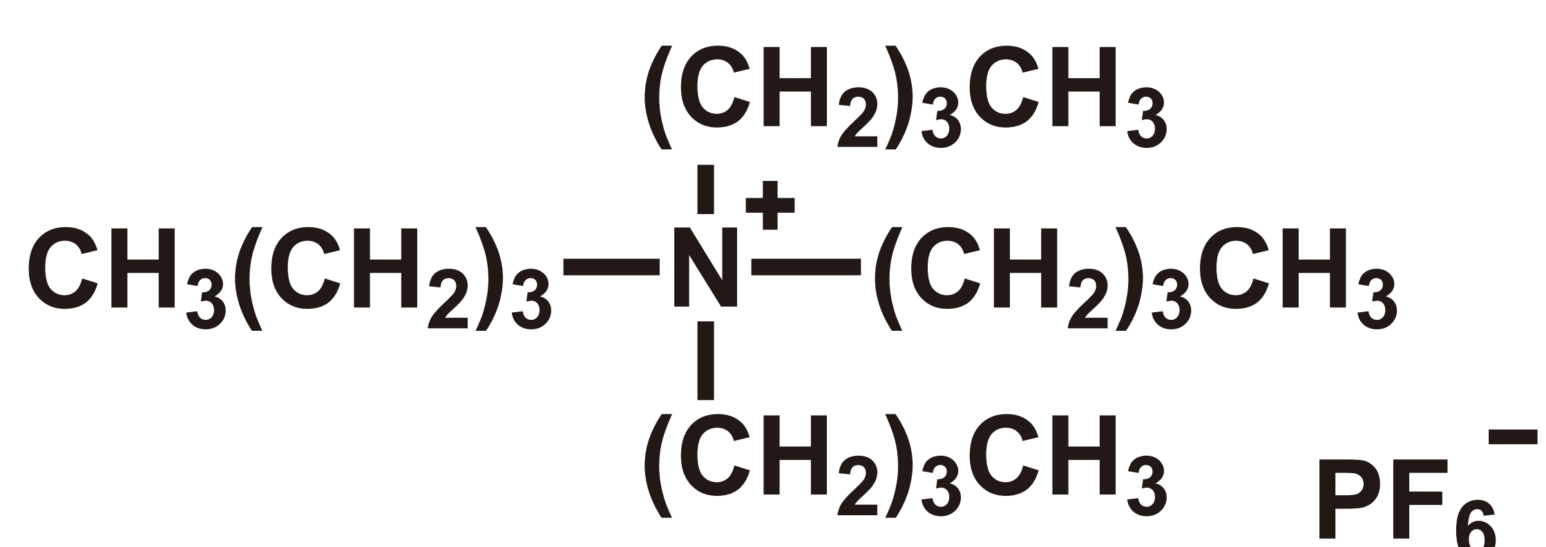
Tetrabutylammonium Hexafluorophosphate [CAS RN: 3109-63-5]
