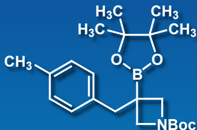
[1-Boc-3-(4-methylbenzyl)azetid-3-yl]boronic Acid Pinacol Ester
