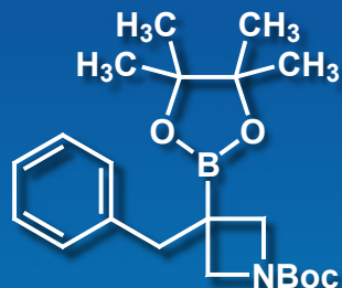
(3-Benzyl-1-Boc-azetid-3-yl)-boronic Acid Pinacol Ester
