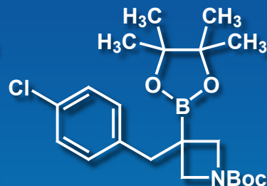
[1-Boc-3-(4-chlorobenzyl)azetid-3-yl]boronic Acid Pinacol Ester
