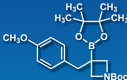
[1-Boc-3-(4-methoxybenzyl)azetid-3-yl]boronic Acid Pinacol Ester
