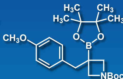
[1-Boc-3-(4-methoxybenzyl)azetidin-3-yl]boronic Acid Pinacol Ester
