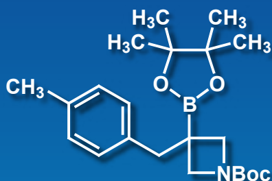
[1-Boc-3-(4-methylbenzyl)azetidin-3-yl]boronic Acid Pinacol Ester
