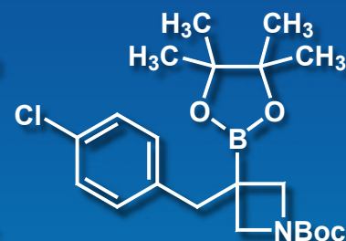
[1-Boc-3-(4-chlorobenzyl)azetidin-3-yl]boronic Acid Pinacol Ester
