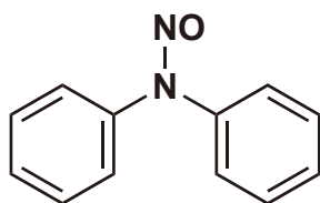
Diphenylnitrosamine
