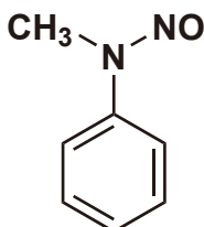
N-Methyl-N-phenylnitrosamine
