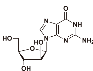
9-β-D-Arabinofuranosyl-guanine Hydrate
