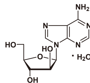
9-(β-D-Arabinofuranosyl)-adenine Monohydrate
