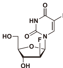
2'-Fluoro-5-iodoarauracil
