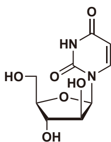
1-β-D-Arabinofuranosyl-uracil
