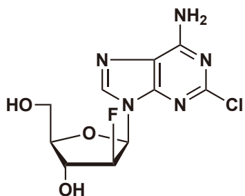
Clofarabine
