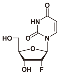
2'-Deoxy-2'-fluorouridine
