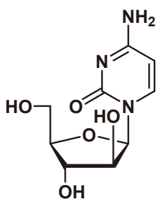
Arabinocytidine
