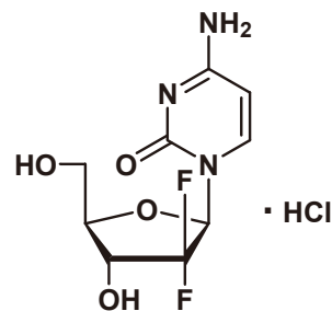
Gemcitabine Hydrochloride
