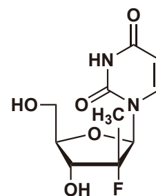
(2'R)-2'-Deoxy-2'-fluoro-2'-methyluridine
