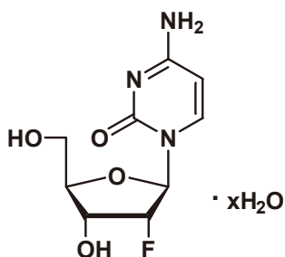
2'-Deoxy-2'-fluorocytidine Hydrate
