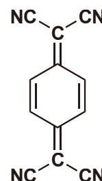
TCNQ 5g / 25g [T0078] TCNQ (purified by sublimation) 1g / 5g [T3034]
