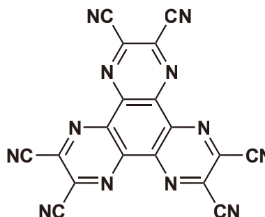
HAT-CN6 200mg / 1g / 5g [D5248]
