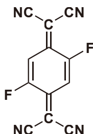
2,5-TCNQF 2 100mg [D3200]
