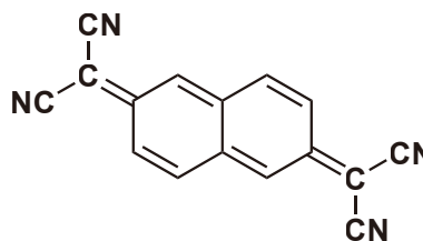
TCNQ 100mg [T1246]
