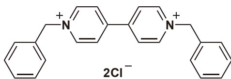
Benzyl Viologen 1g / 5g [D2137]
