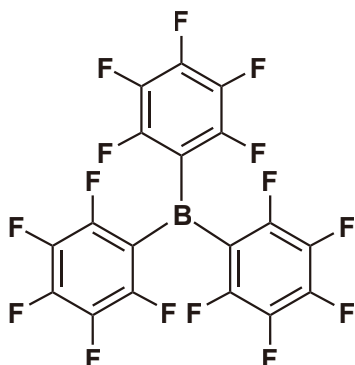
Tris(pentafluorophenyl)borane 1g / 5g [T2313]
