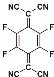
F 4 TCNQ (purified by sublimation) 100mg / 1g [T1131]
