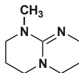
MTBD 1g / 5g [M1443]
