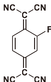
FTCNQ 100mg [F0509]
