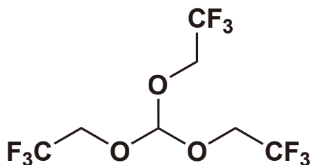
Tris(2,2,2-trifluoroethyl)orthoformate
