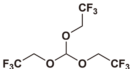
Tris(2,2,2-trifluoroethyl)orthoformate
