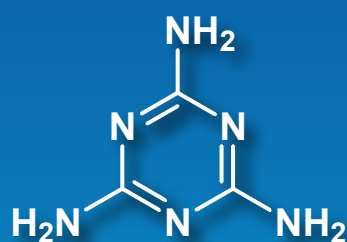
Melamine Monomer
