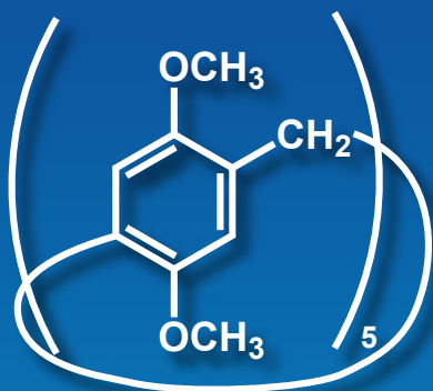
Dimethoxypillar[5]arene
