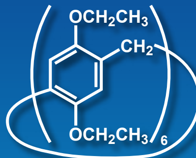
Diethoxypillar[6]arene
