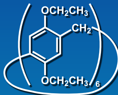
Diethoxypillar[6]arene
