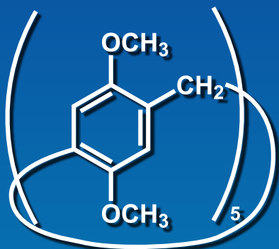
Dimethoxypillar[5]arene
