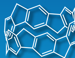
Methylene-bridged [6]cycloparaphenylene
