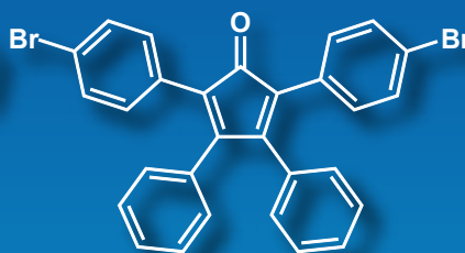
2,5-Bis(4-bromophenyl)- 3,4-diphenylcyclopenta- 2,4-dienone
