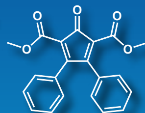
2,5-Bis(methoxycarbonyl)- 3,4-diphenyl- cyclopentadienone
