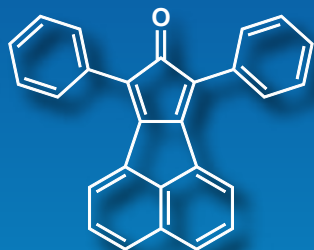
7,9-Diphenyl-8H-cyclopenta- [a]acenaphthylen-8-one
