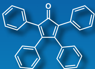
Tetraphenyl- cyclopentadienone
