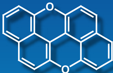
peri-Xanthenoxanthene
