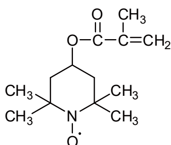
Redox Polymer
