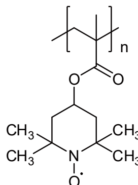
Magnetic Polymer
