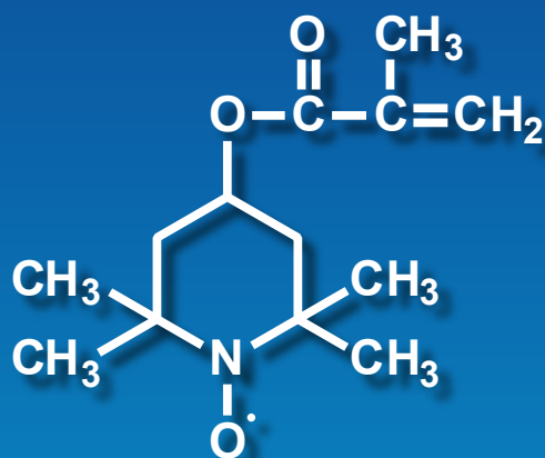
TEMPO Methacrylate
